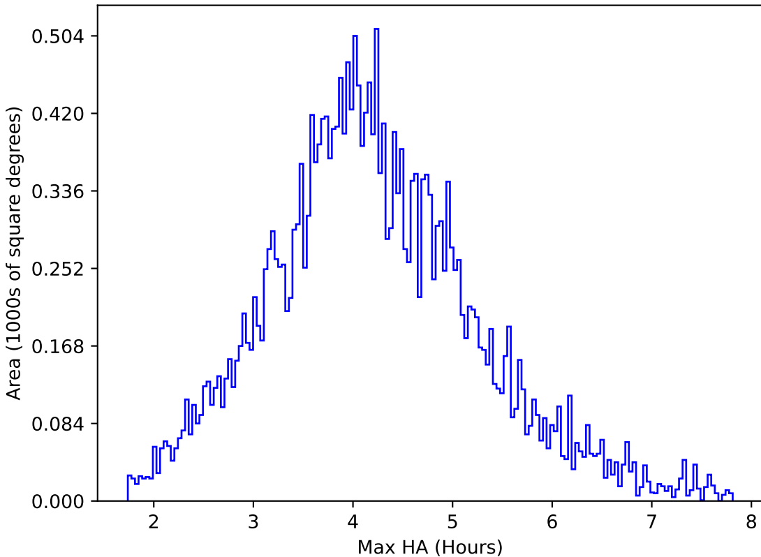
too_elab_r64_d3_griz_v3.4_10yrs All sky r band: Max HA
