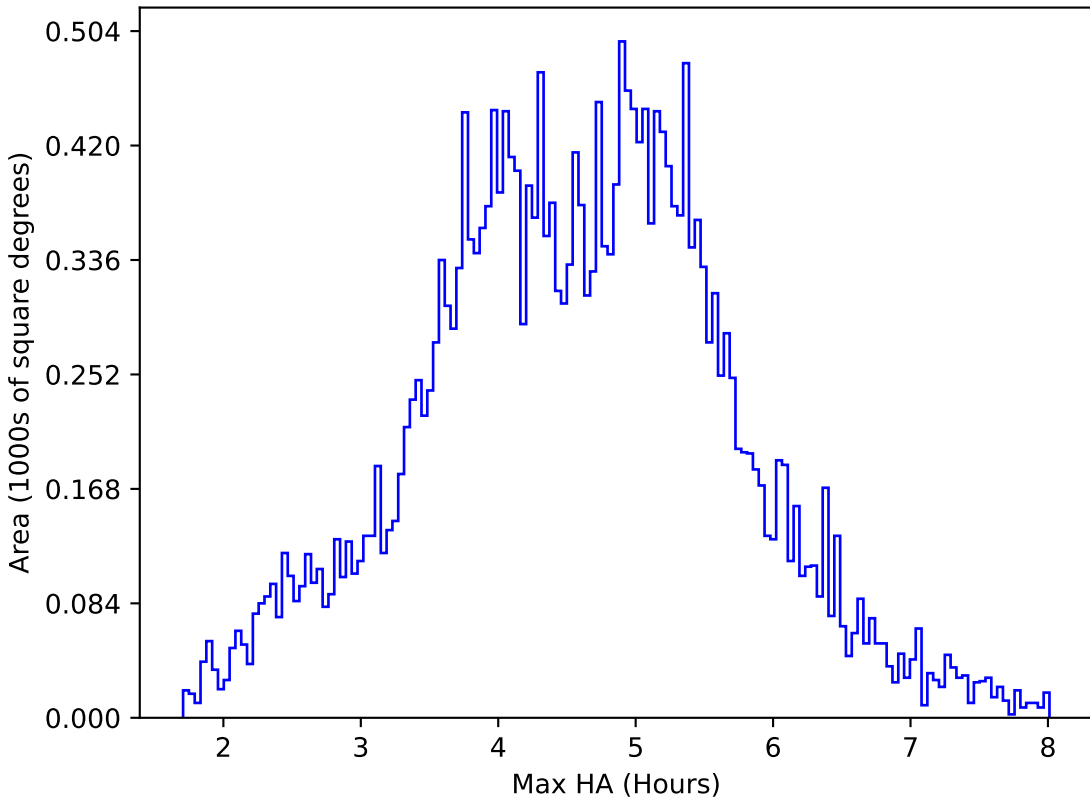
too_elab_r64_d3_griz_v3.4_10yrs All sky i band: Max HA
