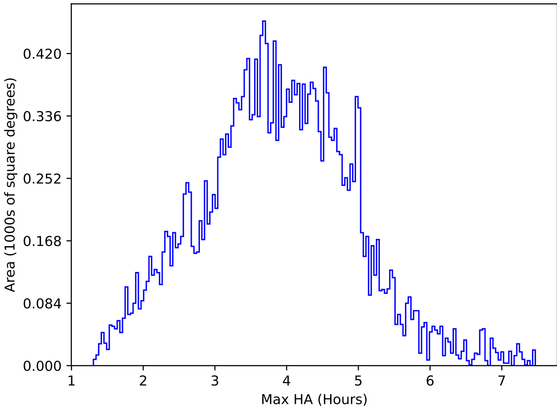
too_elab_r64_d3_griz_v3.4_10yrs All sky g band: Max HA
