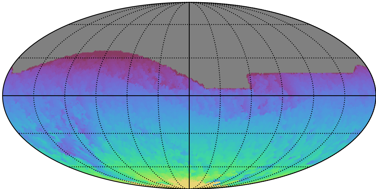
too_elab_r64_d3_griz_v3.4_10yrs All sky all bands: Max HA
