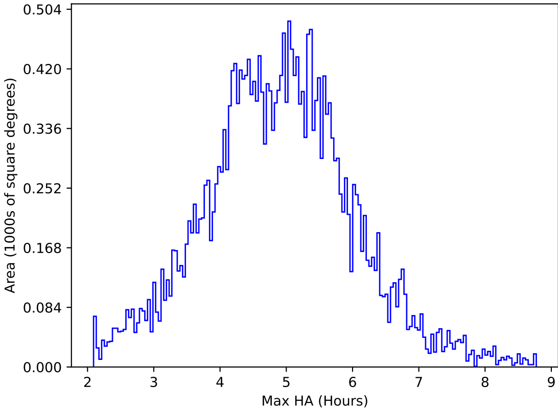
too_elab_r64_d3_griz_v3.4_10yrs All sky all bands: Max HA
