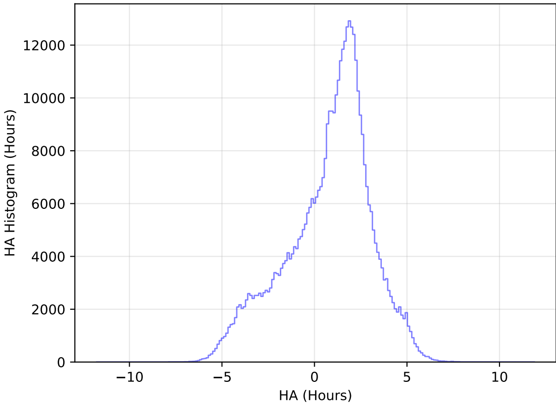
too_elab_r64_d3_griz_v3.4_10yrs WFD z band: HA Histogram
