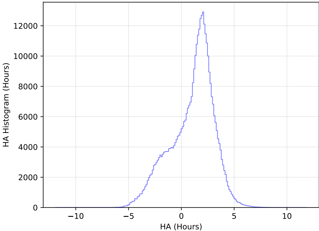
too_elab_r64_d3_griz_v3.4_10yrs WFD y band: HA Histogram
