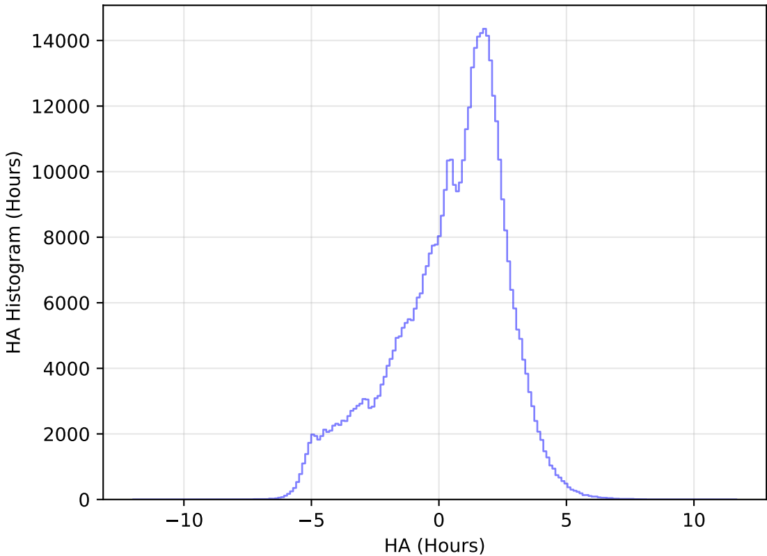
too_elab_r64_d3_griz_v3.4_10yrs WFD r band: HA Histogram
