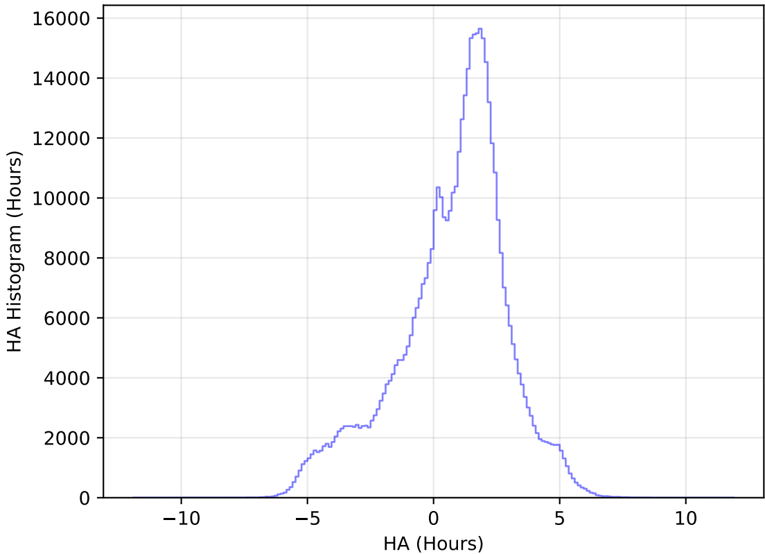
too_elab_r64_d3_griz_v3.4_10yrs WFD i band: HA Histogram
