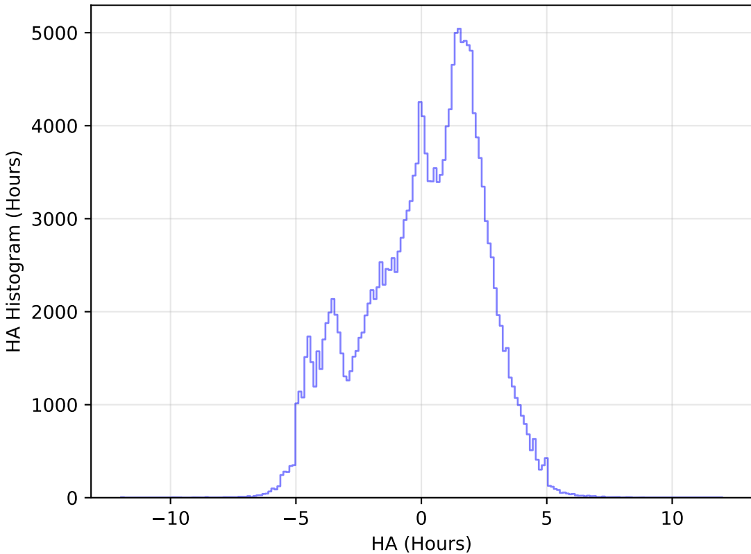
too_elab_r64_d3_griz_v3.4_10yrs WFD g band: HA Histogram
