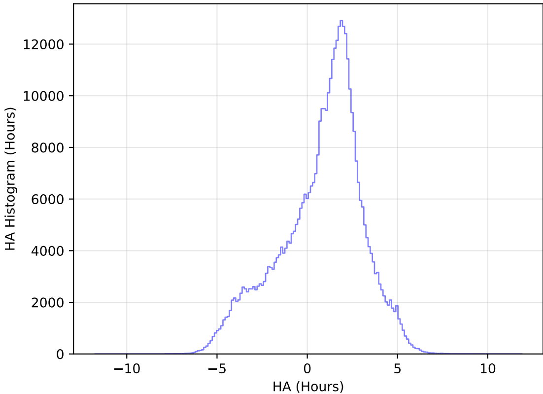
too_elab_r64_d3_griz_v3.4_10yrs All sky z band: HA Histogram
