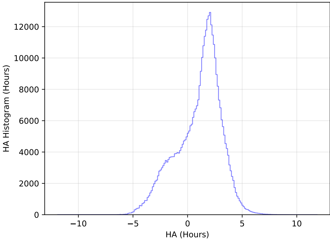
too_elab_r64_d3_griz_v3.4_10yrs All sky y band: HA Histogram
