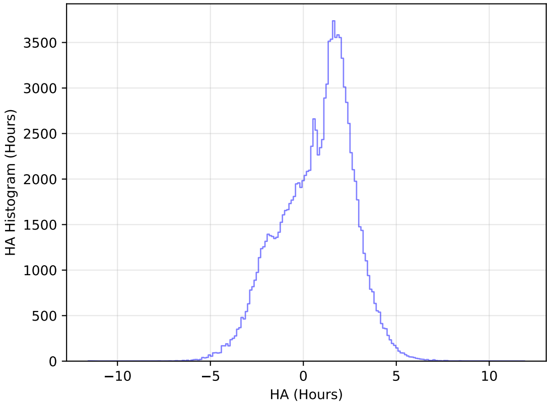
too_elab_r64_d3_griz_v3.4_10yrs All sky u band: HA Histogram
