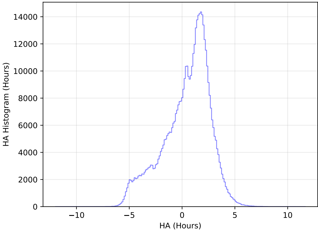
too_elab_r64_d3_griz_v3.4_10yrs All sky r band: HA Histogram
