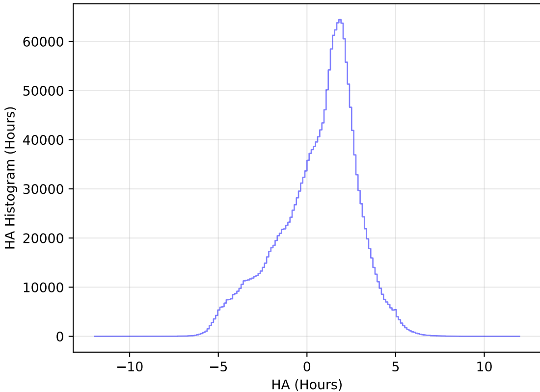
too_elab_r64_d3_griz_v3.4_10yrs All sky all bands: HA Histogram
