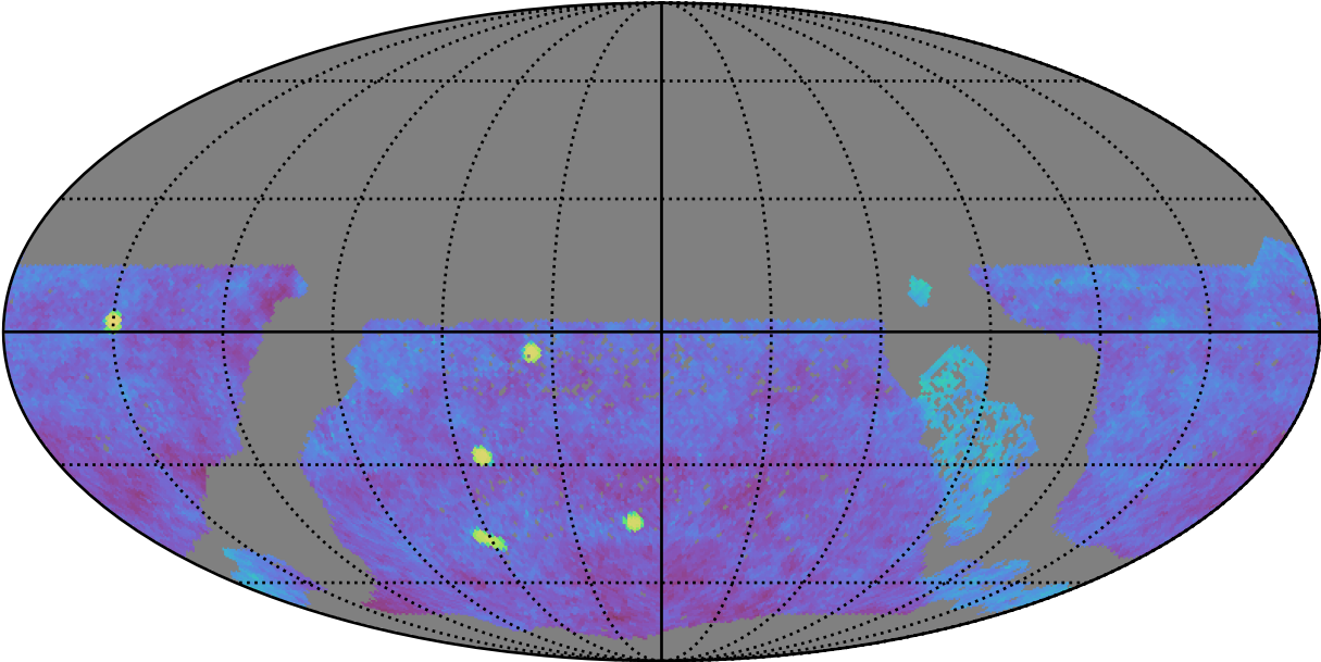
too_elab_r64_d3_griz_v3.4_10yrs gri WFD: Fraction of visits in pairs (10-60 min)
