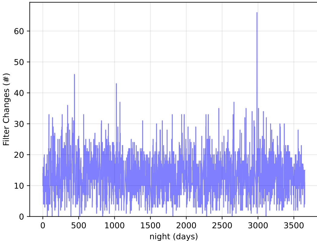
too_elab_r64_d3_griz_v3.4_10yrs Per Night: Filter Changes
