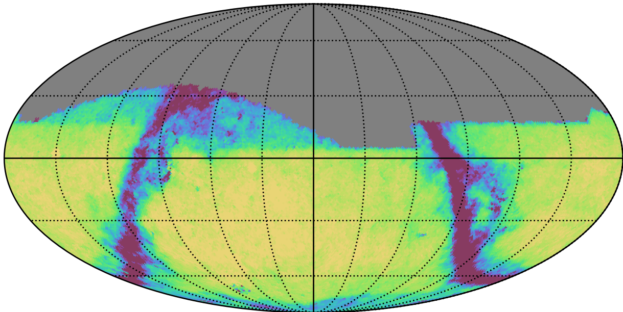
too_elab_r64_d3_griz_v3.4_10yrs Yr 1 r band: Exgal_CoaddM5
