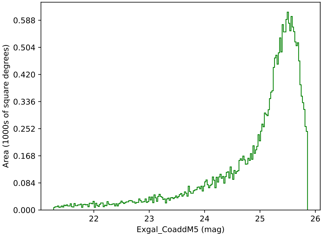
too_elab_r64_d3_griz_v3.4_10yrs Yr 1 g band: Exgal_CoaddM5
