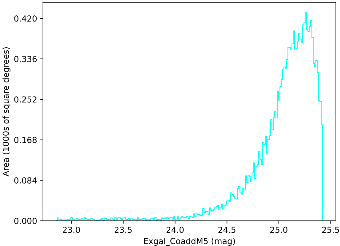
too_elab_r64_d3_griz_v3.4_10yrs WFD u band: Exgal_CoaddM5
