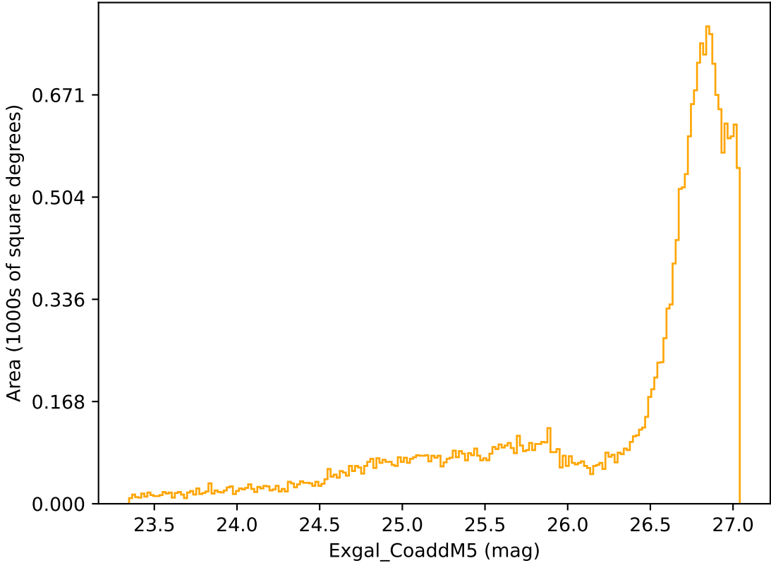
too_elab_r64_d3_griz_v3.4_10yrs All sky r band: Exgal_CoaddM5
