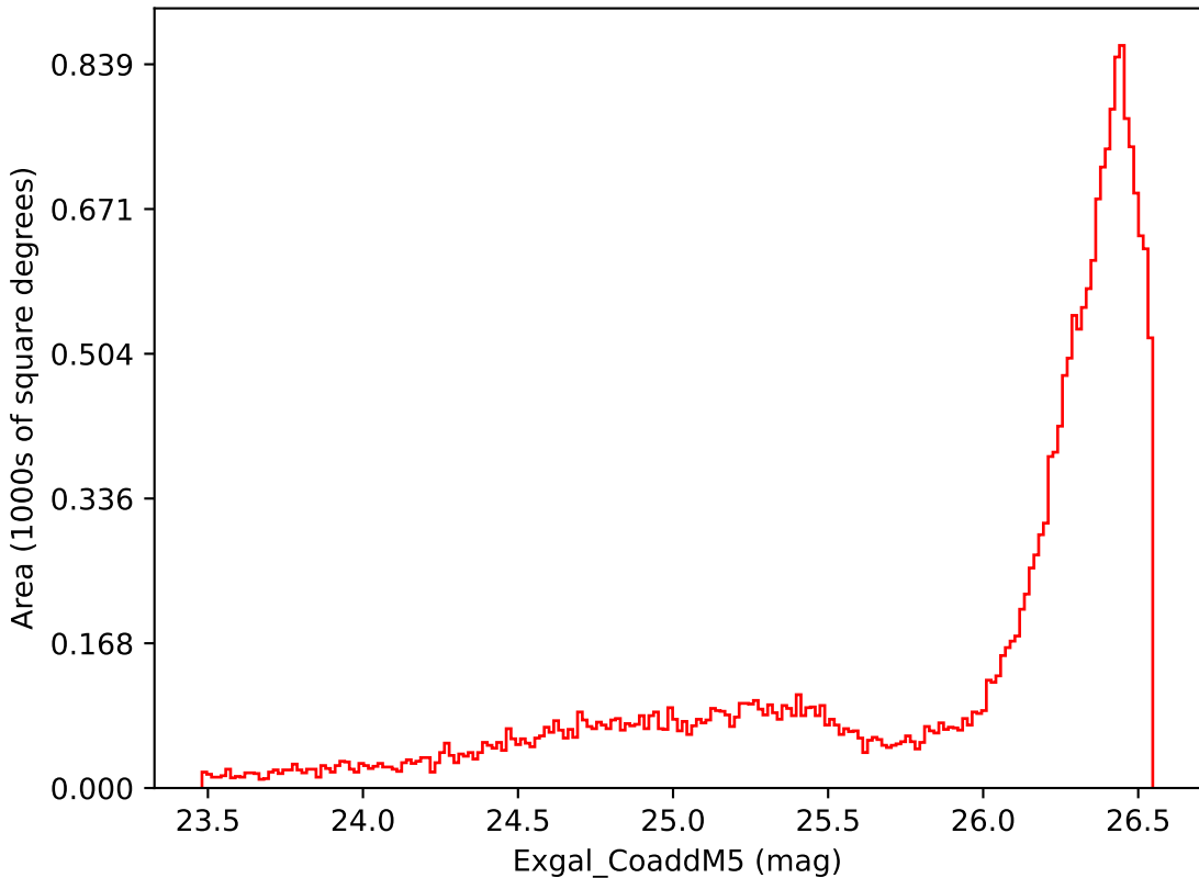
too_elab_r64_d3_griz_v3.4_10yrs All sky i band: Exgal_CoaddM5
