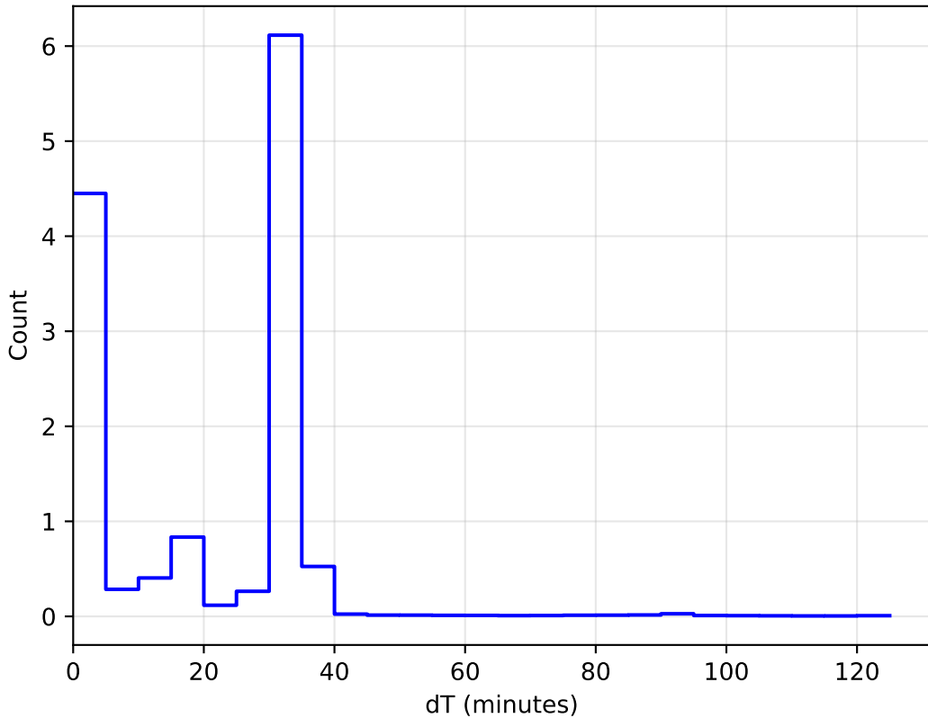
too_elab_r64_d3_griz_v3.4_10yrs All sky: DeltaT Histogram 1e6
