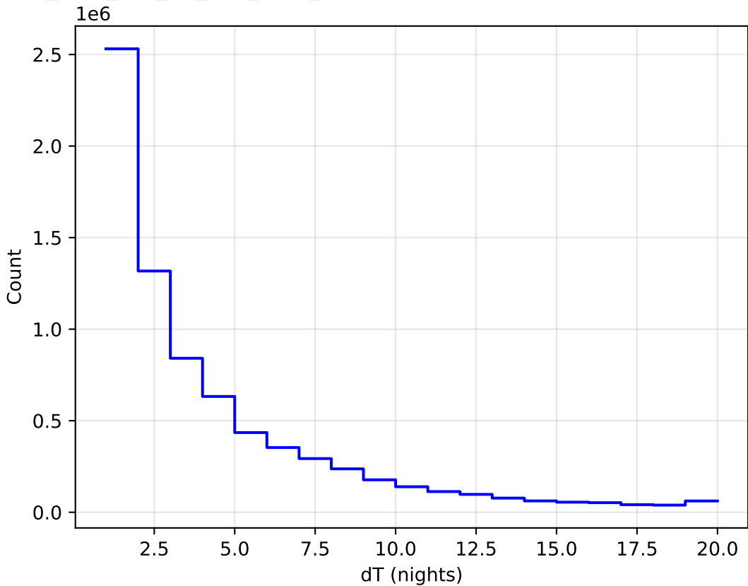
too_elab_r64_d3_griz_v3.4_10yrs WFD all bands: DeltaNight Histogram
