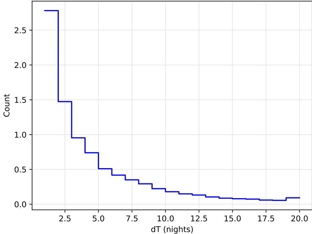
too_elab_r64_d3_griz_v3.4_10yrs All sky all bands: DeltaNight Histogram
