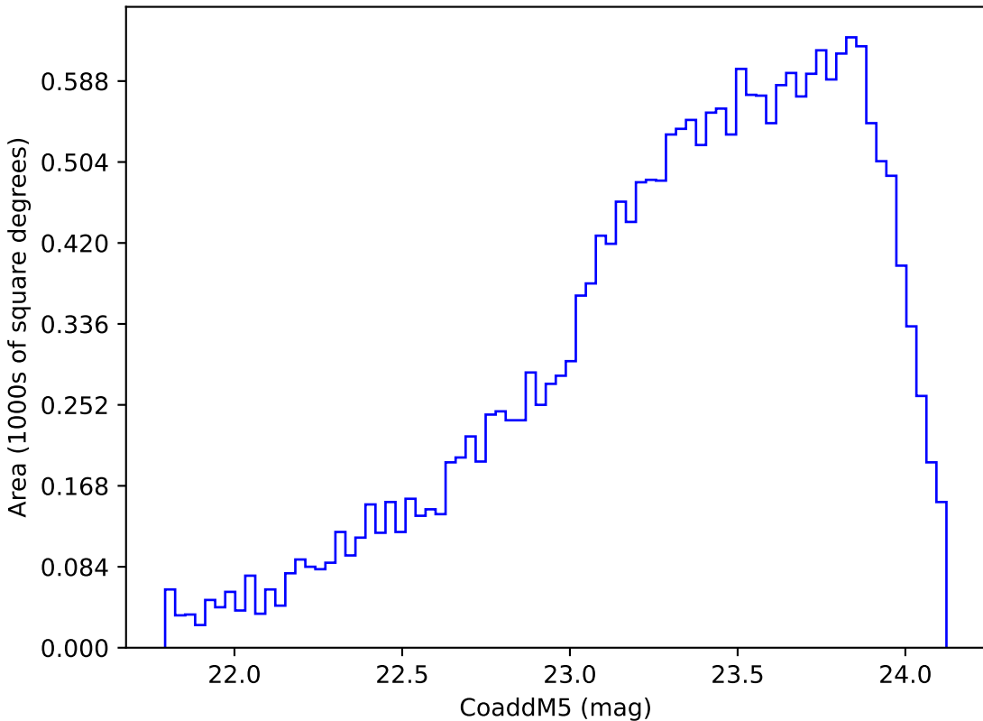
too_elab_r64_d3_griz_v3.4_10yrs Yr 3-4 y band: CoaddM5
