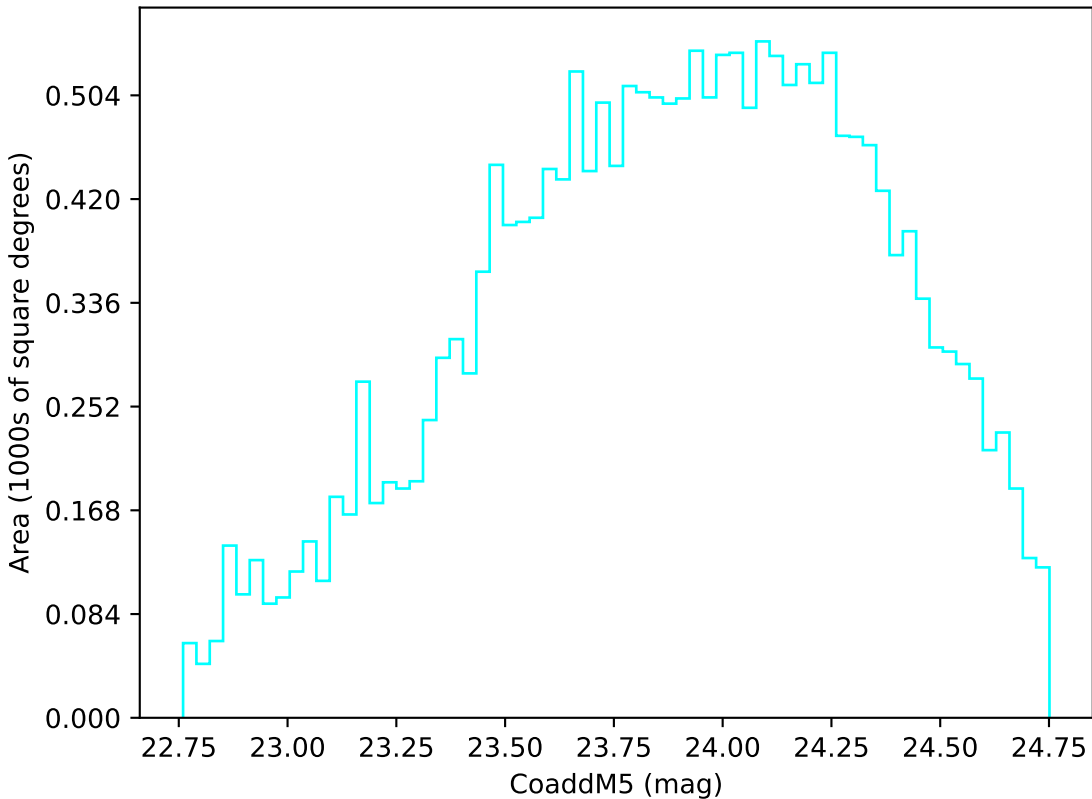
too_elab_r64_d3_griz_v3.4_10yrs Yr 3-4 u band: CoaddM5
