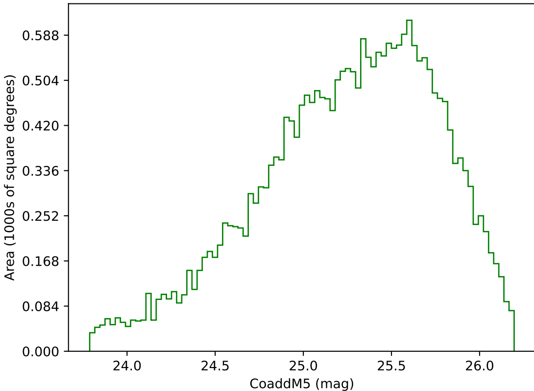
too_elab_r64_d3_griz_v3.4_10yrs Yr 3-4 g band: CoaddM5
