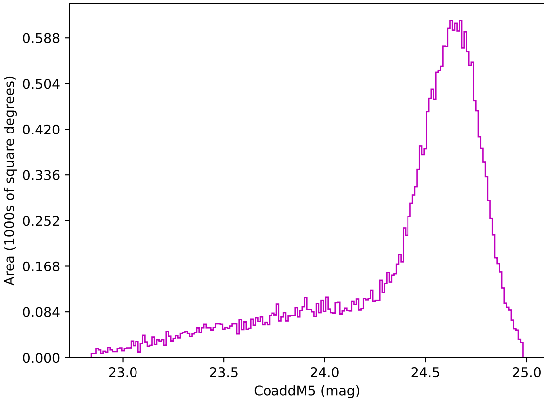
too_elab_r64_d3_griz_v3.4_10yrs Yr 1 z band: CoaddM5
