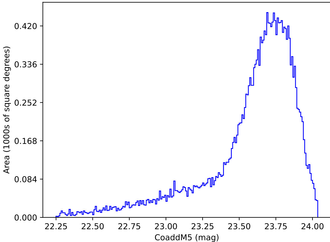
too_elab_r64_d3_griz_v3.4_10yrs Yr 1 y band: CoaddM5
