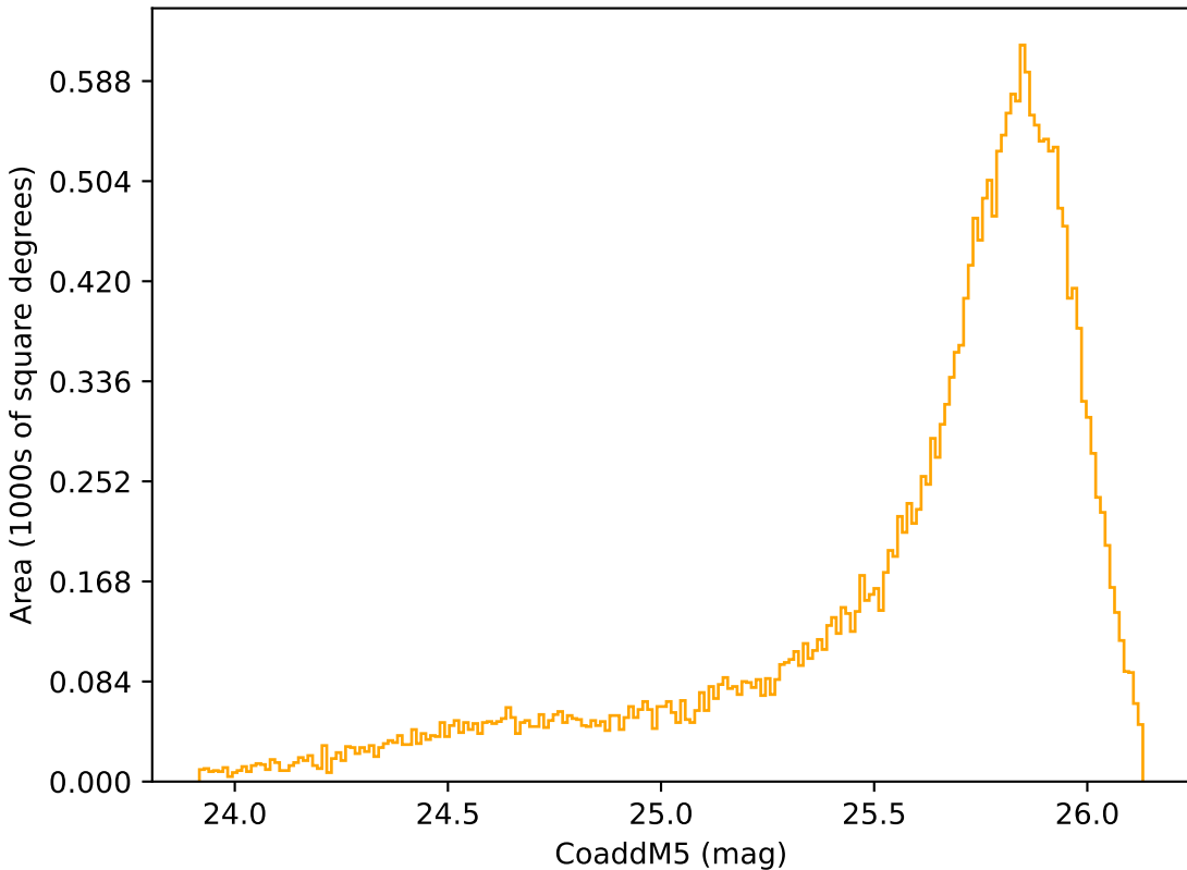
too_elab_r64_d3_griz_v3.4_10yrs Yr 1 r band: CoaddM5
