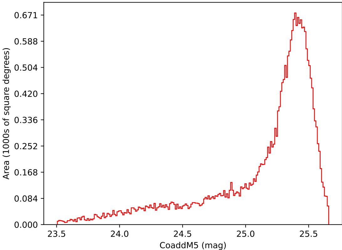
too_elab_r64_d3_griz_v3.4_10yrs Yr 1 i band: CoaddM5
