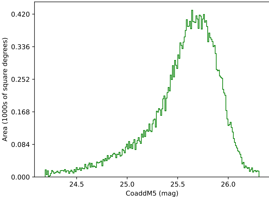
too_elab_r64_d3_griz_v3.4_10yrs Yr 1 g band: CoaddM5
