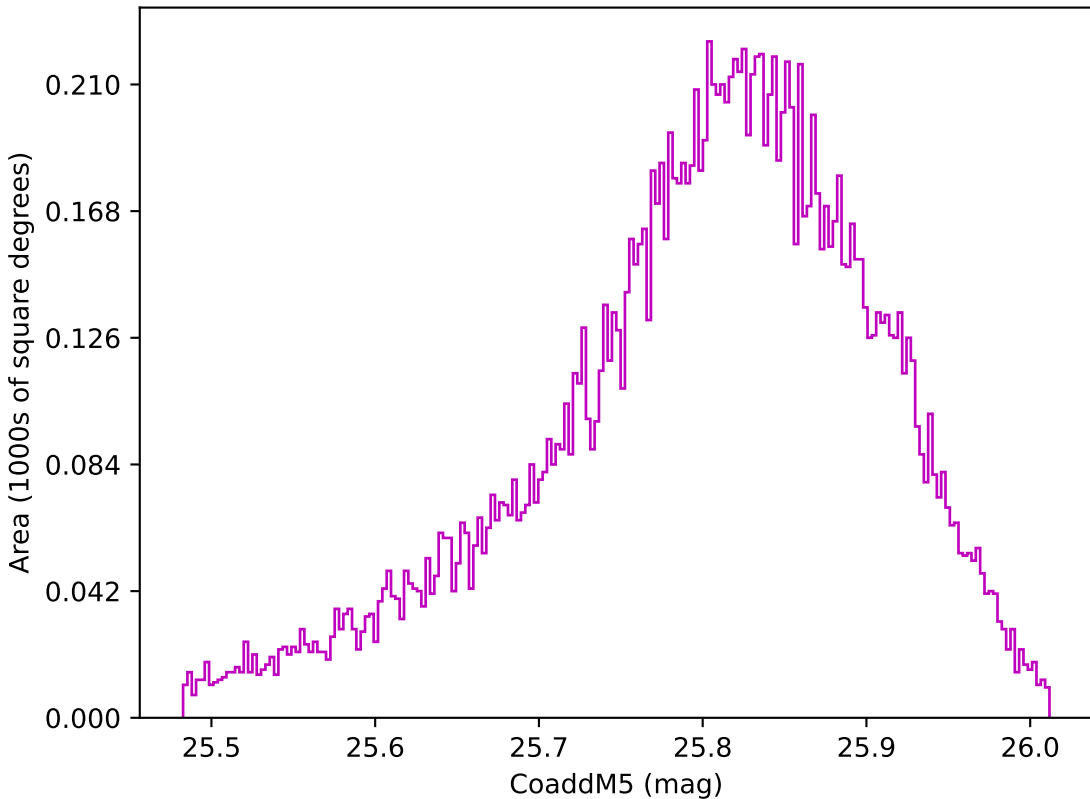
too_elab_r64_d3_griz_v3.4_10yrs WFD z band: CoaddM5
