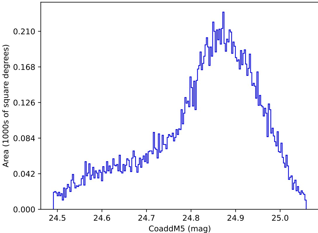
too_elab_r64_d3_griz_v3.4_10yrs WFD y band: CoaddM5
