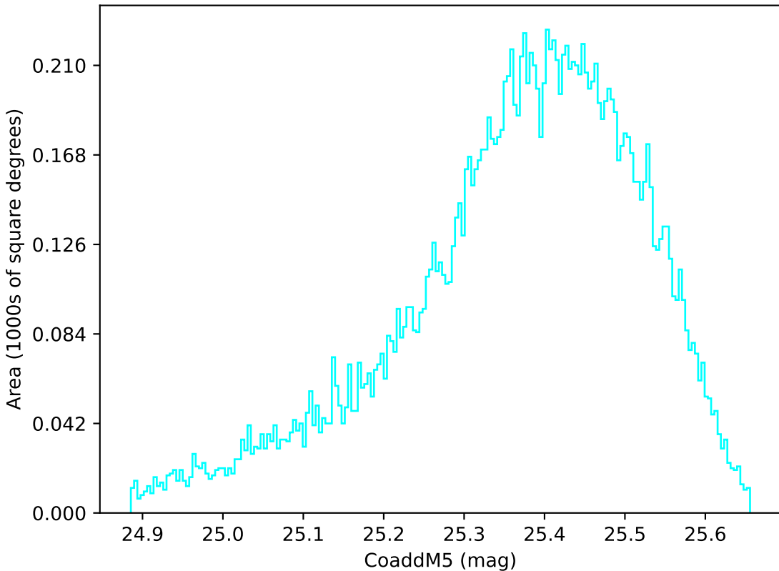
too_elab_r64_d3_griz_v3.4_10yrs WFD u band: CoaddM5
