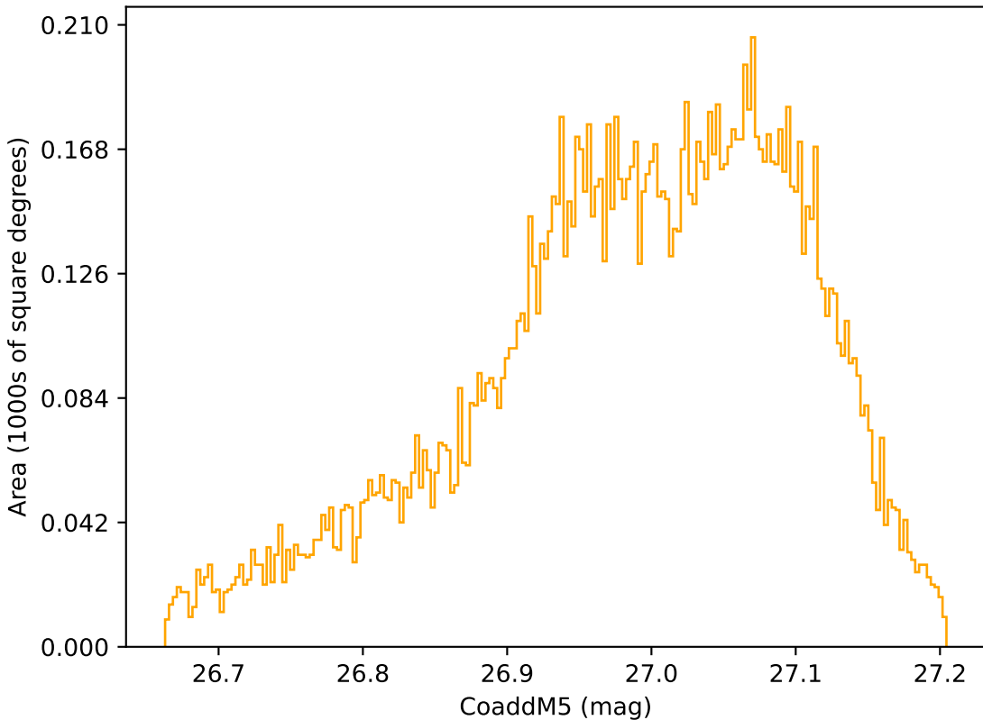
too_elab_r64_d3_griz_v3.4_10yrs WFD r band: CoaddM5
