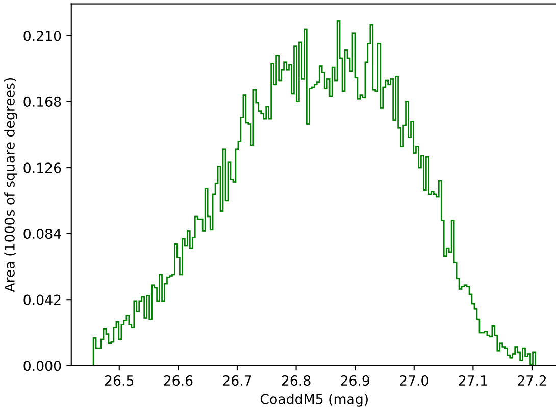
too_elab_r64_d3_griz_v3.4_10yrs WFD g band: CoaddM5
