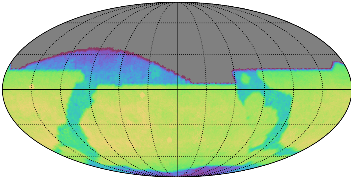
too_elab_r64_d3_griz_v3.4_10yrs All sky z band: CoaddM5
