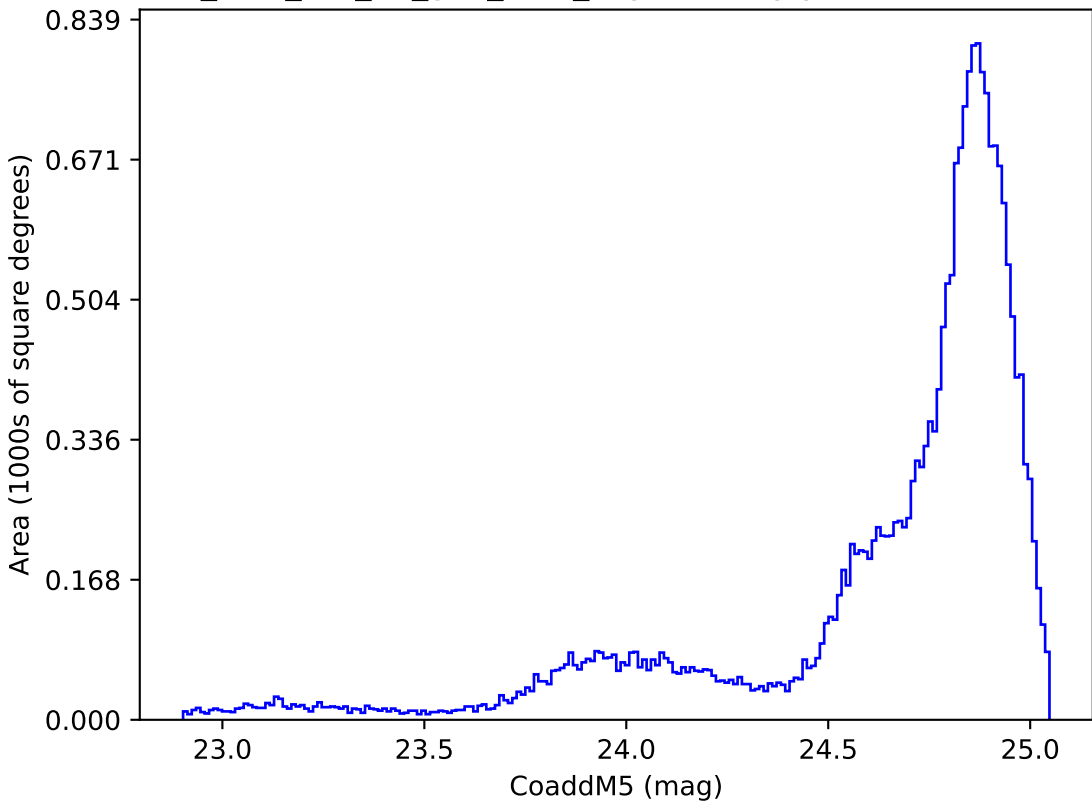
too_elab_r64_d3_griz_v3.4_10yrs All sky y band: CoaddM5
