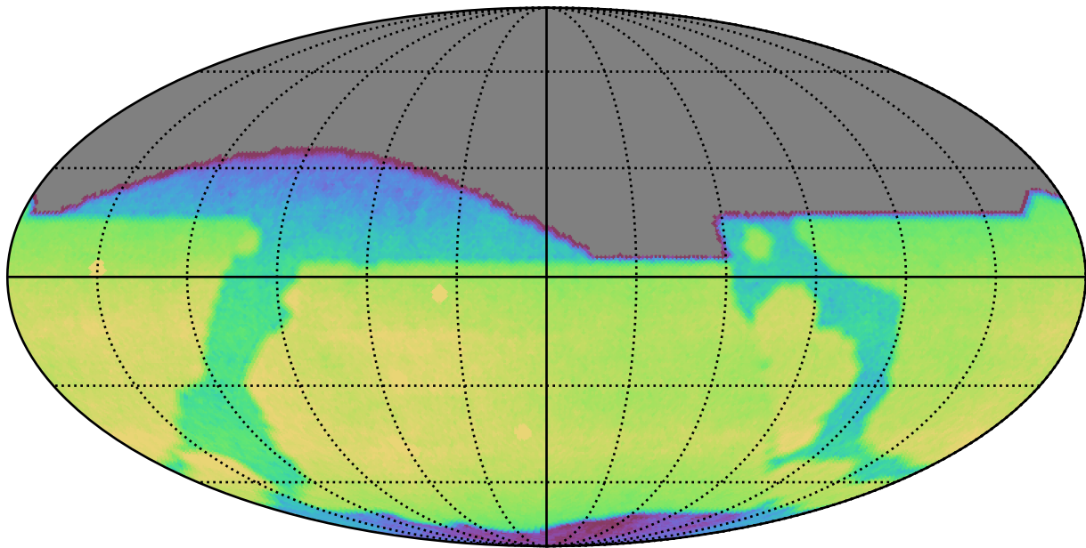
too_elab_r64_d3_griz_v3.4_10yrs All sky r band: CoaddM5
