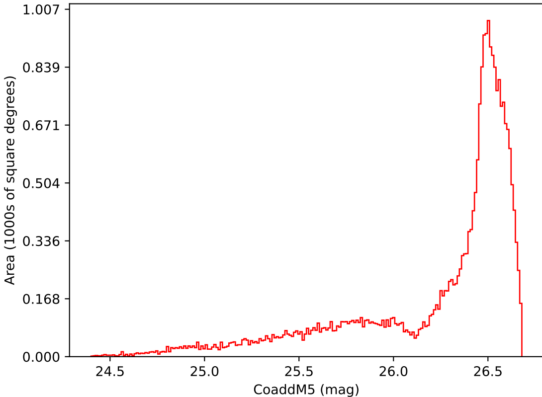
too_elab_r64_d3_griz_v3.4_10yrs All sky i band: CoaddM5
