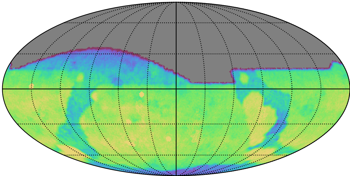
too_elab_r64_d3_griz_v3.4_10yrs All sky g band: CoaddM5
