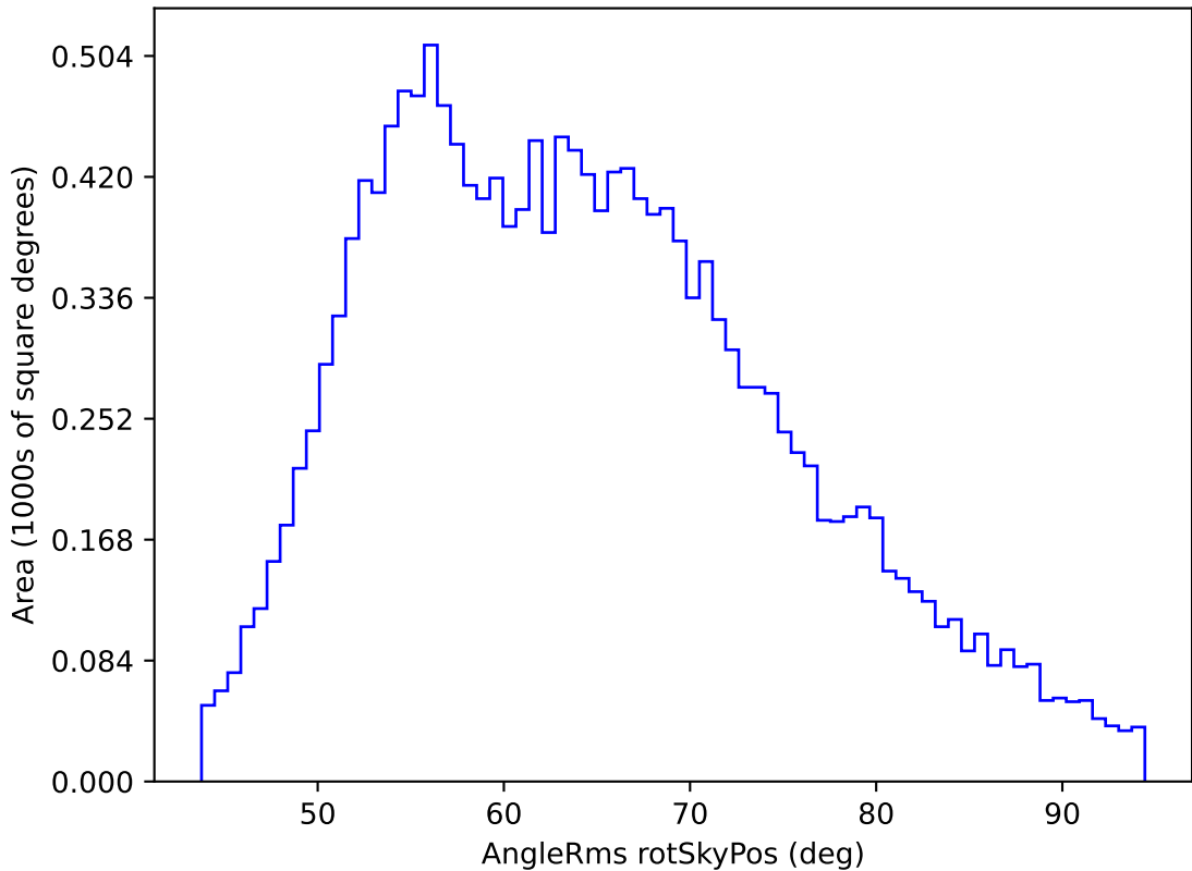
too_elab_r64_d3_griz_v3.4_10yrs WFD u band: AngleRms rotSkyPos
