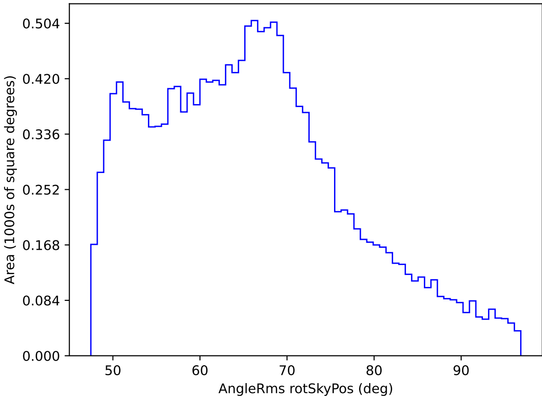
too_elab_r64_d3_griz_v3.4_10yrs WFD r band: AngleRms rotSkyPos
