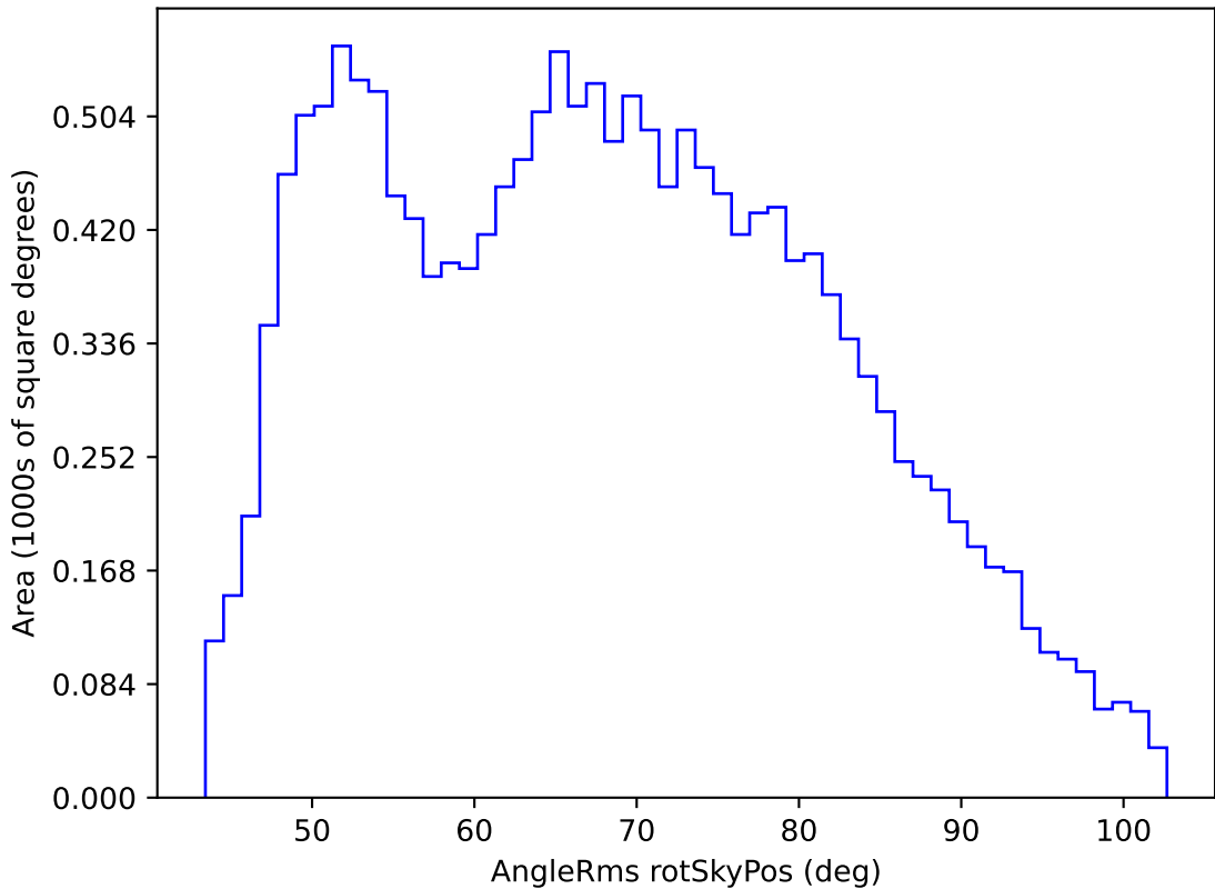
too_elab_r64_d3_griz_v3.4_10yrs WFD g band: AngleRms rotSkyPos
