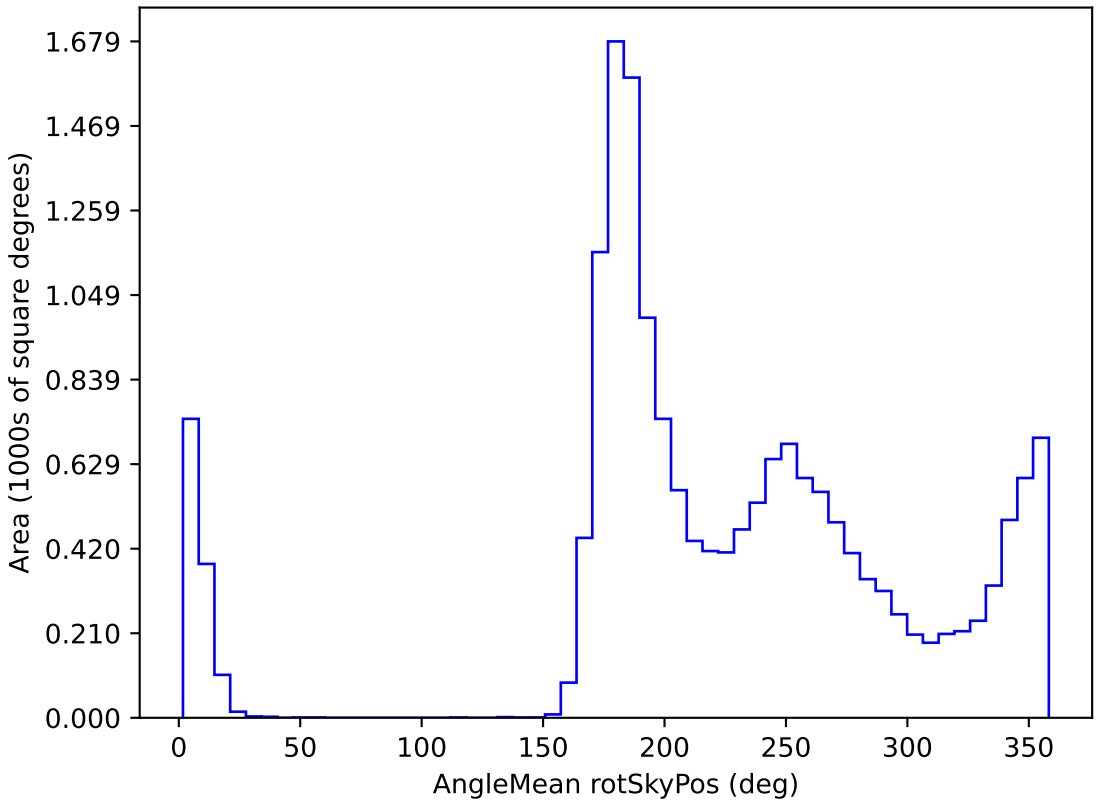
too_elab_r64_d3_griz_v3.4_10yrs WFD y band: AngleMean rotSkyPos
