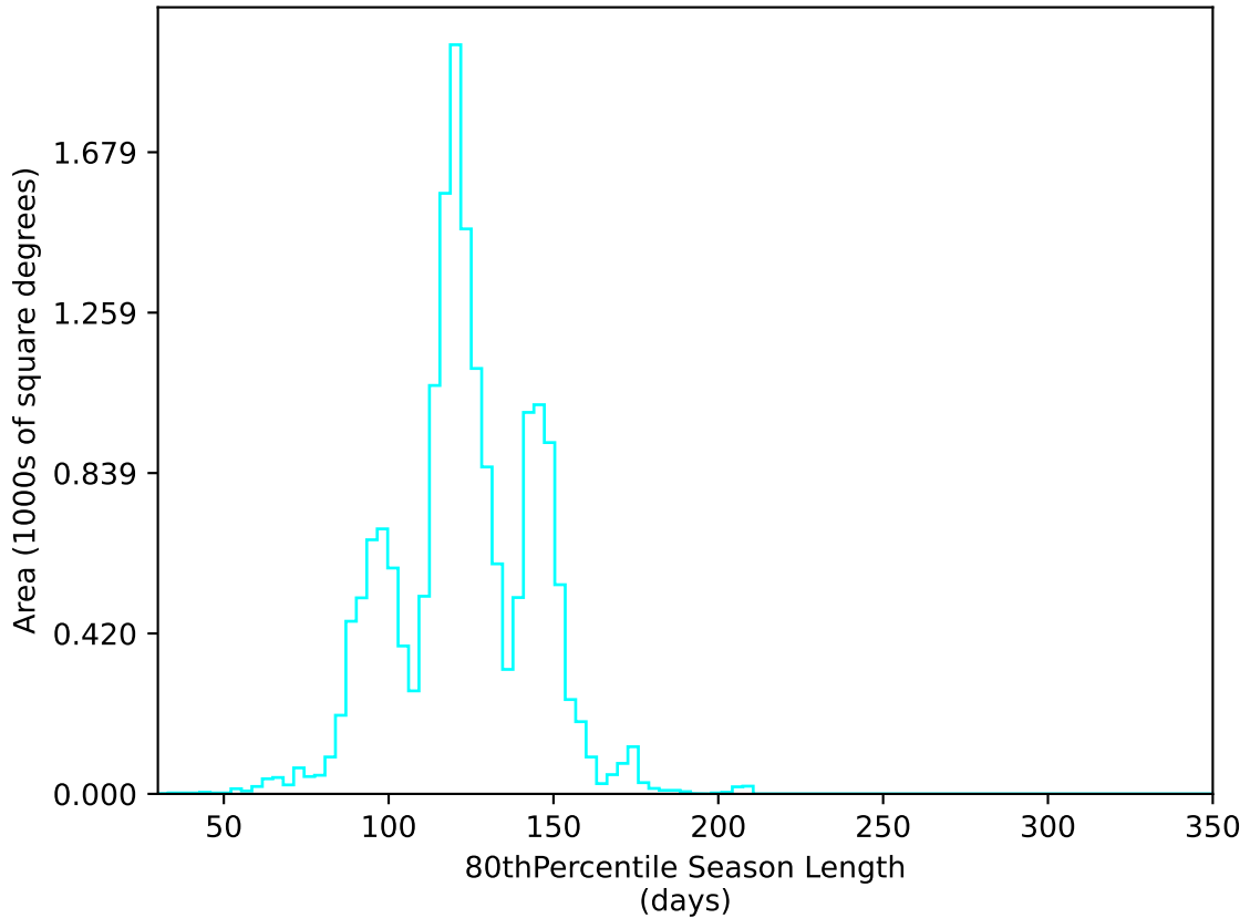
too_elab_r64_d3_griz_v3.4_10yrs WFD u band: 80thPercentile Season Length
