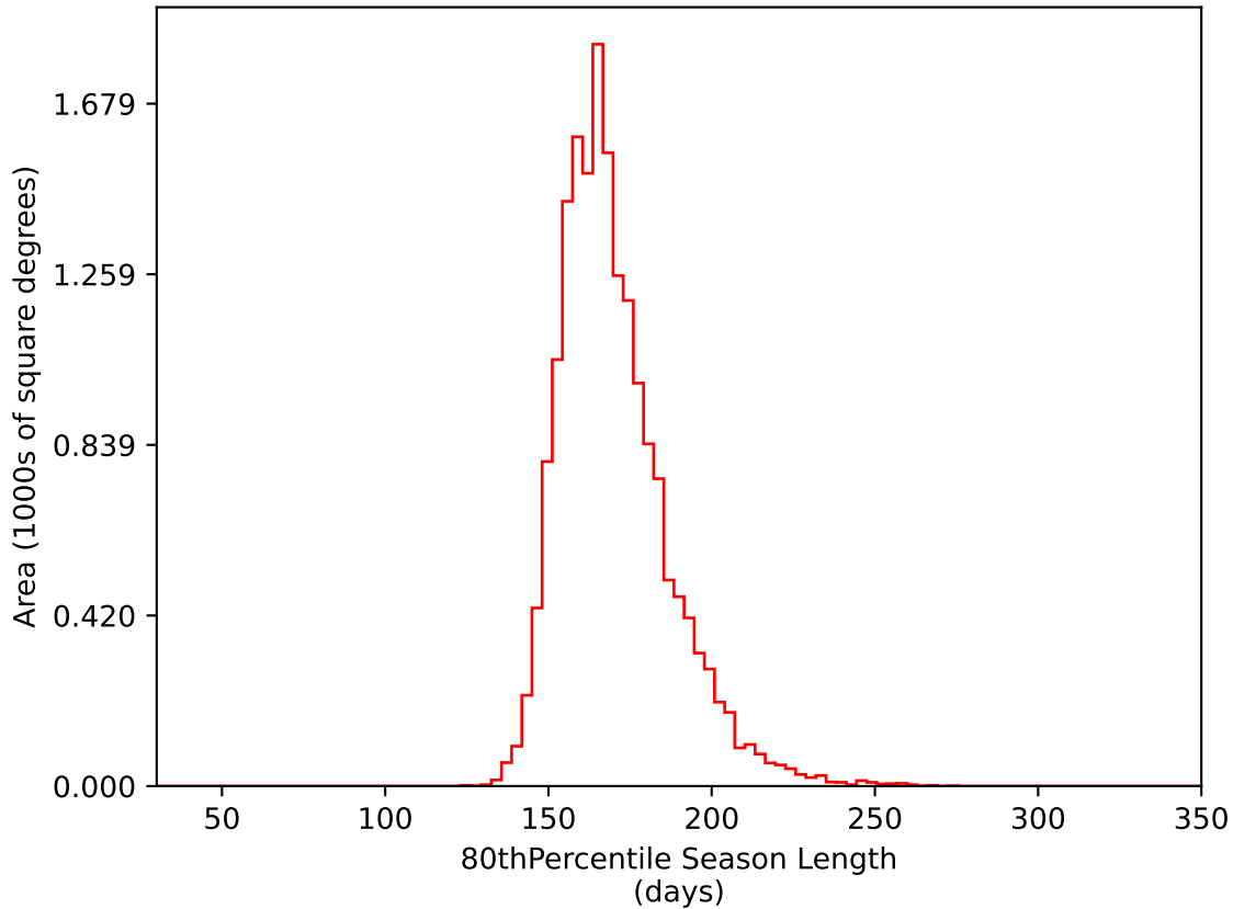
too_elab_r64_d3_griz_v3.4_10yrs WFD i band: 80thPercentile Season Length
