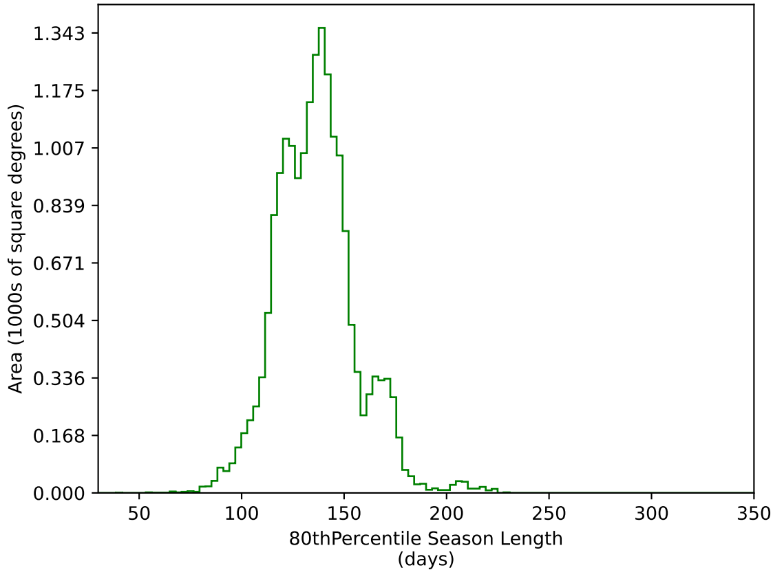
too_elab_r64_d3_griz_v3.4_10yrs WFD g band: 80thPercentile Season Length
